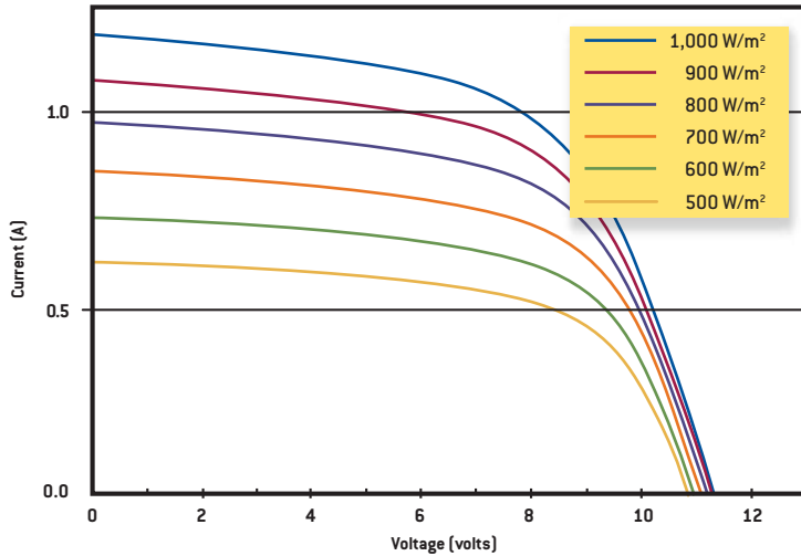
Power Plastic 620 Solar Charger: IV Curves
